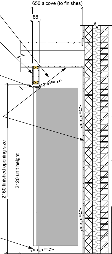
Section through enclosed housing ( 1 : 25 )
